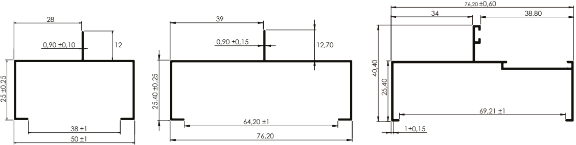
CANAL 2" x 1" 2" x 1" Channel
