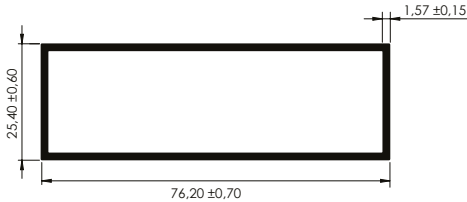
TUBULAR 3" x 1" x 0.062" 3"x 1"x 0.062" Hollow Tube
