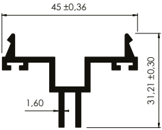
PISAVIDRIO Glass Holder
