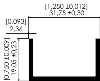
CANAL 1.25" x 0.75" x 0.093" 1.25" x 0.75" x 0.093" Channel
