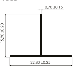
TEE CIELO RASO Low Ceiling Tee
