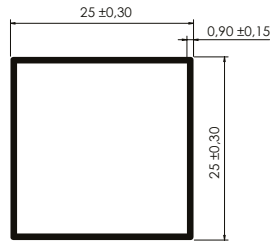
TUBO 1" 1" Hollow Tube
