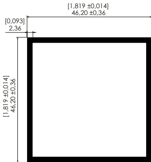
TUBULAR 1.8" X 1.8" X 0.093" 1.8" x 1.8" x 0.093" Hollow Tube
