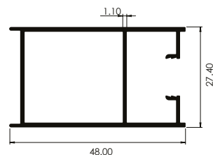
HOJA LATERAL Side Rail
