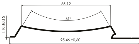
ENCHAPE CURVO Curved Veneer
