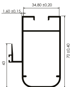
HOJA CENTRAL REDONDA Rounded Interlocker
