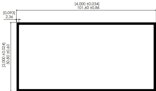
TUBULAR 4" X 2" 4" x 2" Hollow Tube
