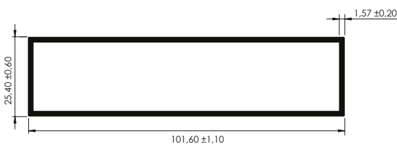
TUBULAR 4" x 1" x 0.062" 4"x 1"x 0.062" Patio Section
