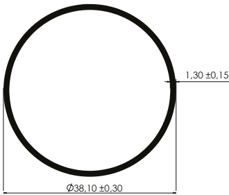
TUBO 1-1/2" 1-1/2" Hollow Tube
