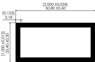
TUBULAR 2" X 1" 2" x 1" Hollow Tube
