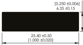
PLATINA DE 1" x 1/4" 1" x 1/4" Plate
