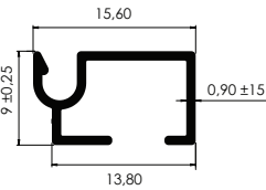
MOSQUITERO Mosquito Net
