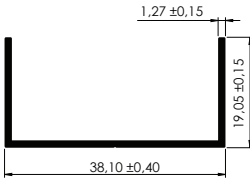
CANAL DE 1-1/2" x 3/4" 1-1/2" x 3/4" Channel
