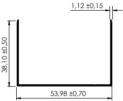
CANAL DE 1 1/2" X 2" 1 1/2" x 2" Rec Channel
