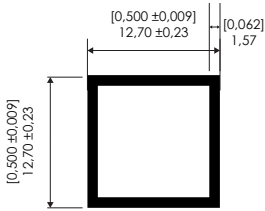
TUBULAR 1/2" x 1/2" x 0.062" 1/2" x 1/2" x 0.062" Hollow Tube
