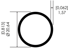
TUBULAR REDONDO 13/16" x 0.062" 13/16" x 0.062" Round Hollow Tube
