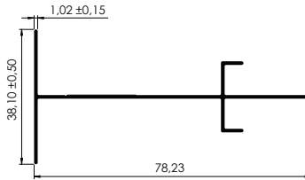
CONECTOR DE PANEL DE 3" 3" Panel Connector
