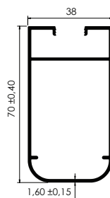
HOJA LATERAL REDONDA Rounded Side Rail
