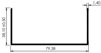
CANAL DE 1 1/2" X 3" 1 1/2" x 3" Rec Channel
