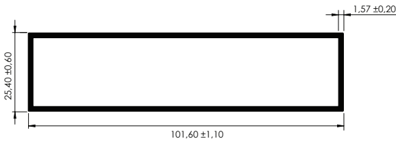
TUBULAR 4" x 1" x 0.062" 4"x 1"x 0.062" Patio Section
