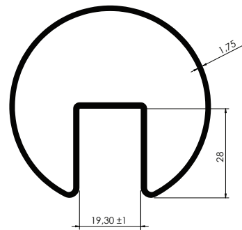
PASAMANOS 2-1/2" 2-1/2" Handrail
