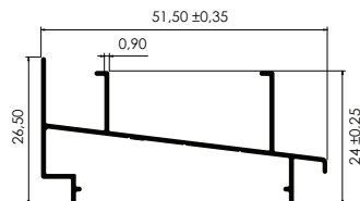
SILLAR Sill
