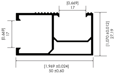
RIEL SOLAR Solar Railing
