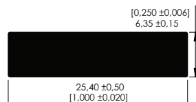
PLATINA DE 1" x 1/4" 1" x 1/4" Plate
