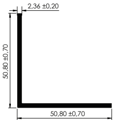
ANGULO 2" x 2" Angle 2"x 2"
