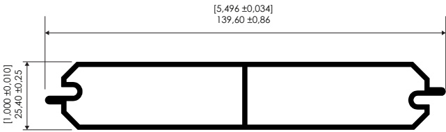
PANEL HORIZONTAL PARA CERCAS Fence Horizontal Panel
