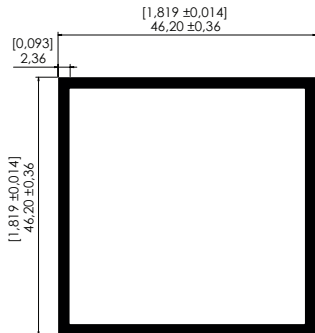
TUBULAR 1.8" X 1.8" X 0.093" 1.8" x 1.8" x 0.093" Hollow Tube
