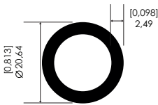
TUBULAR REDONDO 13/16" x 0.098" 13/16" x 0.098" Round Hollow Tube
