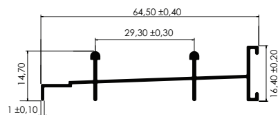
SILLAR Sill
