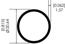
TUBULAR REDONDO 13/16" x 0.062" 13/16" x 0.062" Round Hollow Tube
