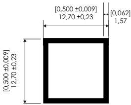
TUBULAR 1/2" x 1/2" x 0.062" 1/2" x 1/2" x 0.062" Hollow Tube
