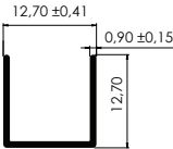
CANAL 1/2" x 1/2" 1/2" x 1/2" Channel
